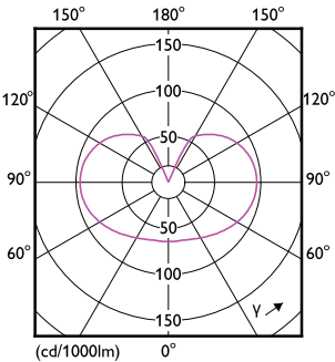
Light Distribution Diagram - LED classic 75W E27 WW A60 FR ND 1CT10
