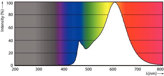
Spectral Power Distribution Colour - LED classic 75W E27 WW A60 FR ND 1CT10
