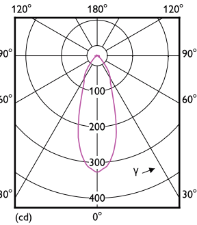
Light Distribution Diagram - CoreProLEDspot ND 3-40W R63 E27 827 36D
